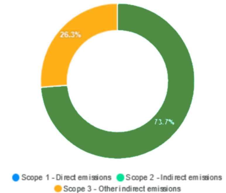
GHG Emissions
